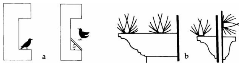
Figure 3. A board or metal covering over a ledge at a 45° angle (a) or porcupine wires (b) can be used to prevent roosting and nesting.
