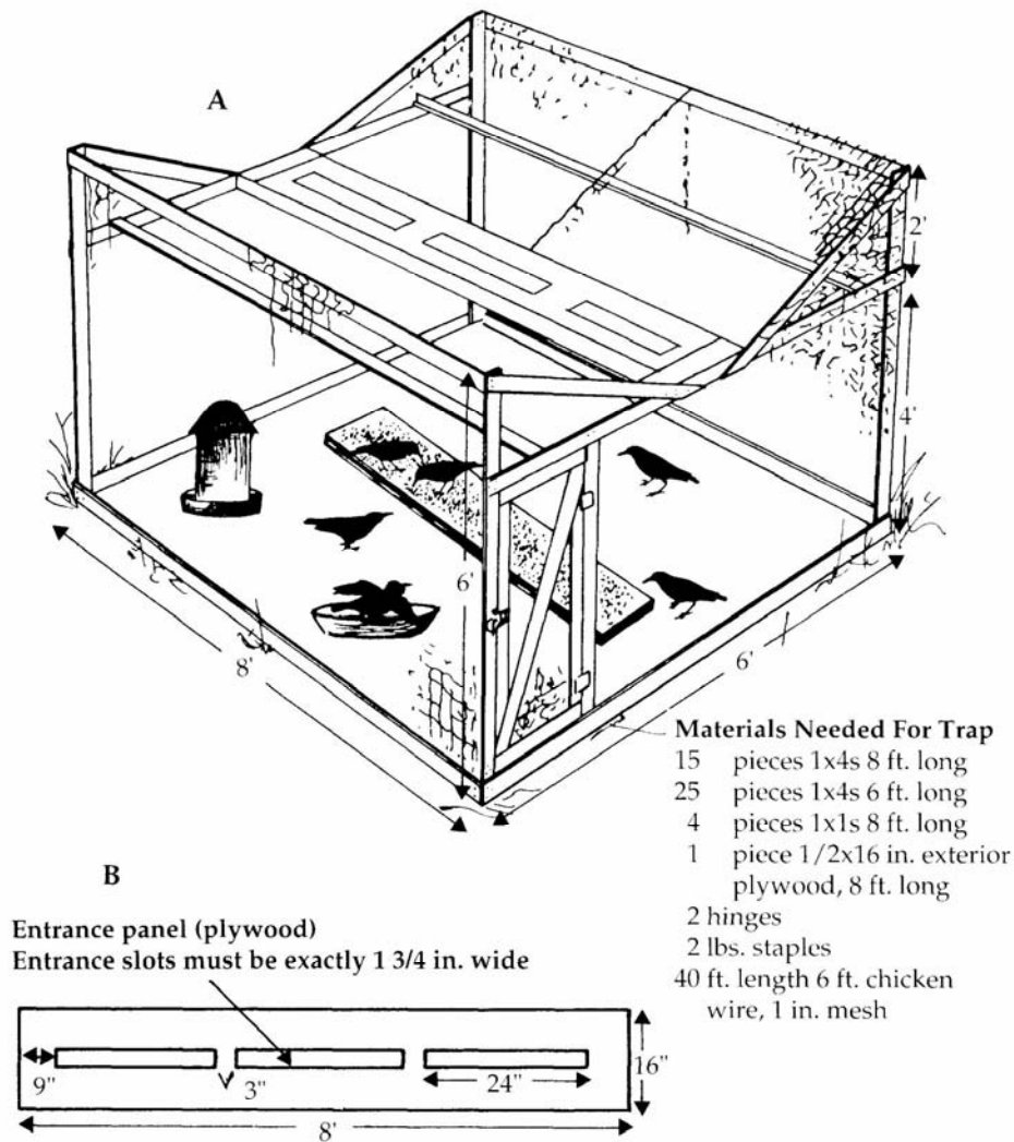
Figure 7. Starling decoy trap: (A) assemble view and (B) details of the entrance panel. Side and end panels are covered with wire on the outside, top panels are covered on the inside of the frame.
